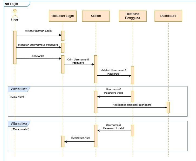
Gambar.5 Sequence Diagram Login
