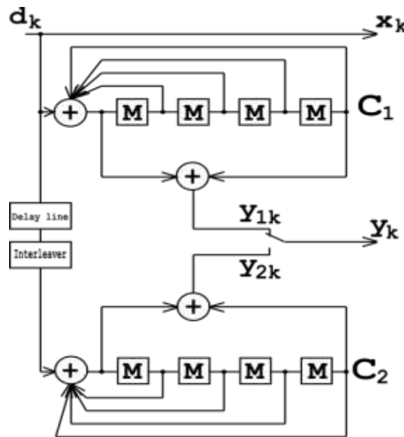
Fig.1 Turbo code encoder
