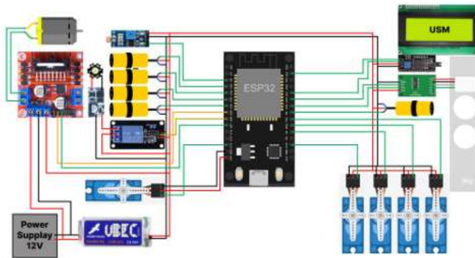
Figure 3. Wiring System
