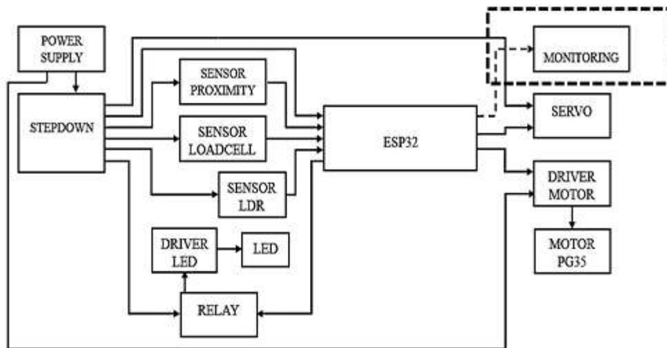
Figure 1. Block Diagram
