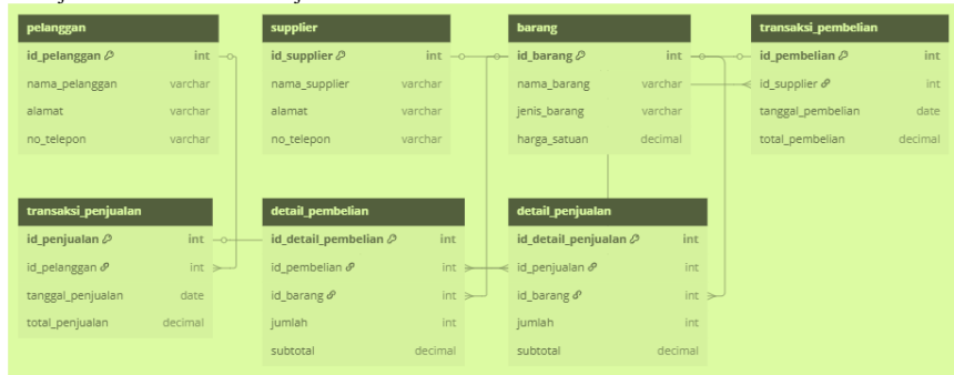
Figure 7. Entity Relationship Diagram (ERD)
