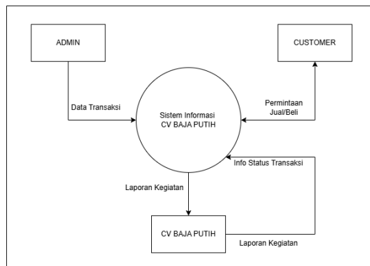
Figure 5. Context Diagram
