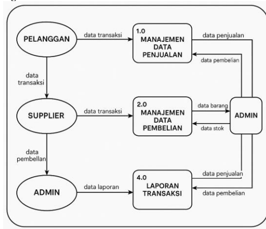
Figure 6. Data Flow Diagram Level 1
