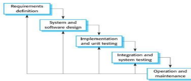
Figure 2. Waterfall
